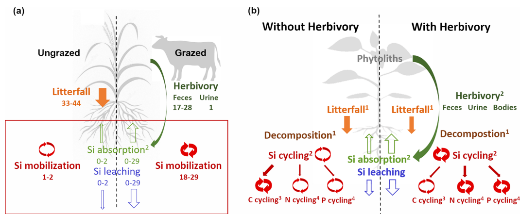
Figure 3. (a) Schematic of Si fluxes ( \text{kg ha}^{-1} \text{ yr}^{-1} ) in hypothetical ungrazed and grazed grassland, dominated by cows, adapted from Vandevenne et al. (2013). Annual net primary production is assumed to be the same for both systems ( 11\,000 \text{ kg ha}^{-1} \text{ yr}^{-1} ), and all biomass is converted to litter or consumed by grazers in the grazed system. A biomass conversion ratio of 1 : 4 for grass versus feces is suggested for all herbivores. Mobilization percentages for faeces are based on ranges (minimum–maximum values) obtained in a dissolution experiment by Vandevenne et al. (2013) after 24 h in rain water; for urine, a conservative estimation of 3 % mobilization was used. (b) Schematic of potential nutrient cycle differences in the plant–soil system with and without herbivory. Size of arrows denotes the size of the flux relative to the alternative scenario. 1 Schaller et al. (2016). 2 Brizuela et al. (1986). 3 Street-Perrott and Barker (2008). 4 Neu et al. (2017), Schaller et al. (2017).
