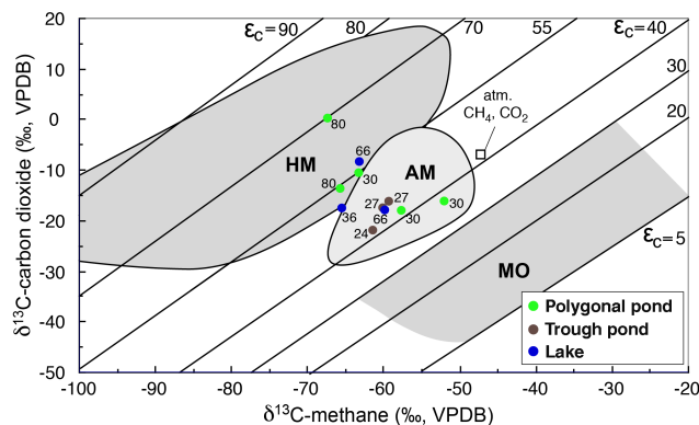
Figure 8. Carbon isotope composition ( \delta^{13}\text{C} ) of \text{CH}_4 (x axis) and \text{CO}_2 (y axis) emitted by the sampled ponds and lakes. HM=hydrogenotrophic methanogenesis; AM=acetoclastic methanogenesis; MO=methane oxidation.
